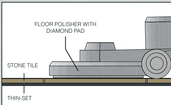
Fig 2. The joints, along with the stone are then honed to create a flush, seamless floor.
