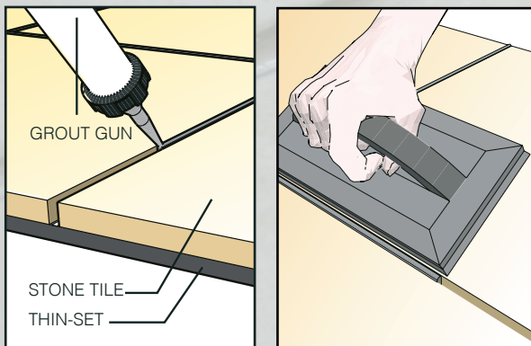
Fig 1. Traditional grout or epoxy grout into joints of a completed installation with a pressurized grout gun or applied directly in the grout joint with a grout float.
